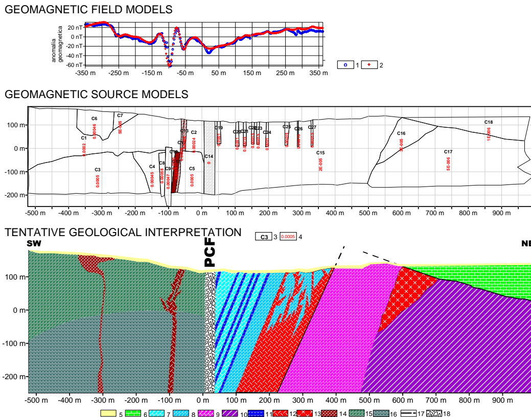
Fig. 4. Tentative interpretative model of the geomagnetic anomaly across PCF:
