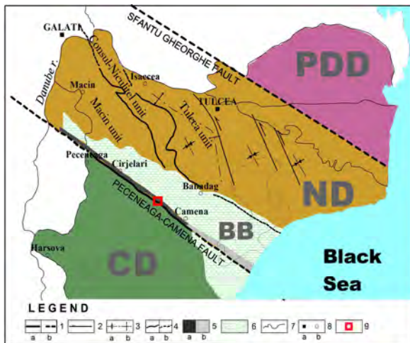
Fig. 1. Simplified tectonic setting of PCF and location of the study area.
