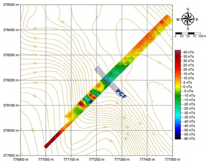
Fig 3. Residual geomagnetic anomaly along various PCF segments (micro-panel P1) as obtained after removing a first order polynomial trend. Black dots mark data points. Brown solid lines show topography contours (in meters). Dashed zone marks the assumed PCF track
