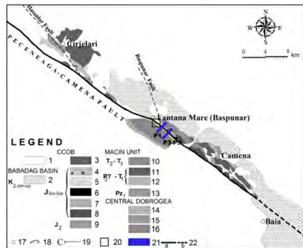
Fig. 2. Simplified geologic sketch of the study area (modified after Grădinaru, 1988).
