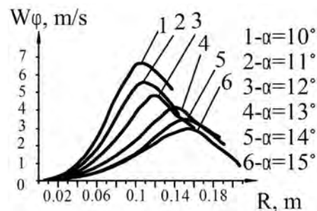
Fig. 4. The calculated change of the circumferential velocity of the granule depending on the angle of the cone opening (at Q = 0.63 \text{ m}^3/\text{s} , z = 0.8 \text{ m} )
