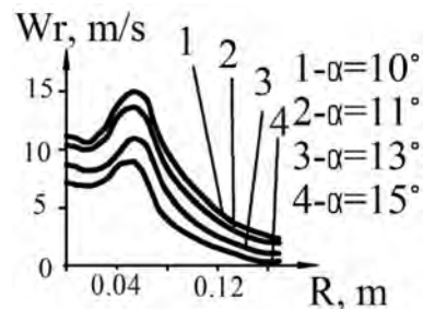
Fig. 6. The calculated change of the radial velocity of the granule depending on the angle of the cone opening (at Q = 0.63 \text{ m}^3/\text{s} , z = 0.8 \text{ m} )
