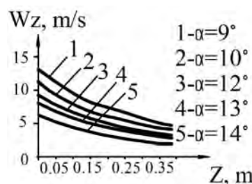
Fig. 8. The calculated change of the longitudinal velocity of the granule throughout the height depending on the angle of the cone opening of the vortex granulator working space (at Q = 0.63 \text{ m}^3/\text{s} )
