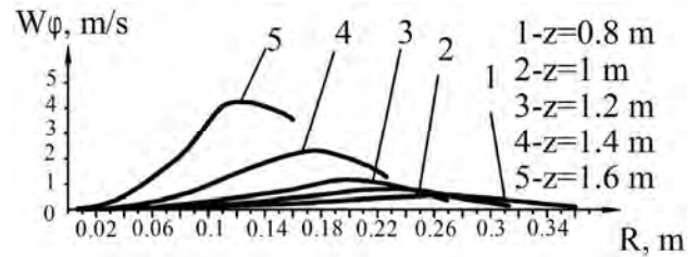
Fig. 2. The calculated change of the circumferential velocity of the granule depending on the height of the working space of the vortex granulator (at \alpha = 13^\circ , Q = 0.63 \text{ m}^3/\text{s} ) at different heights of the device
