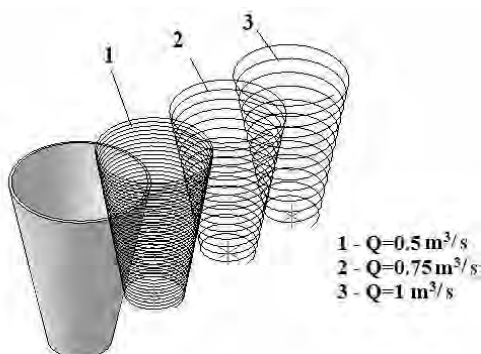
Fig. 9. Effect of the gas flow rate on the trajectory of the granules in the vortex granulator (at \alpha = 13^\circ , d = 3 \text{ mm} , V_{\varphi 0} = 10 \text{ m/s} )
