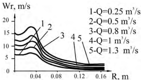
Fig. 5. The calculated change of the radial velocity of the granule depending on the gas flow rate (at \alpha = 13^\circ , z = 0.8 \text{ m} )
