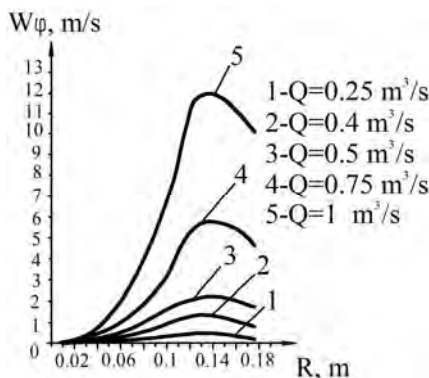
Fig. 3. The calculated change of the circumferential velocity of the granule depending on the gas flow rate (at \alpha = 13^\circ , z = 0.8 \text{ m} )
