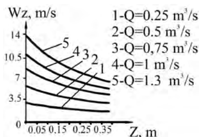
Fig. 7. The calculated change of the longitudinal velocity of the granule throughout the height depending on the gas flow rate (at \alpha = 13^\circ )
