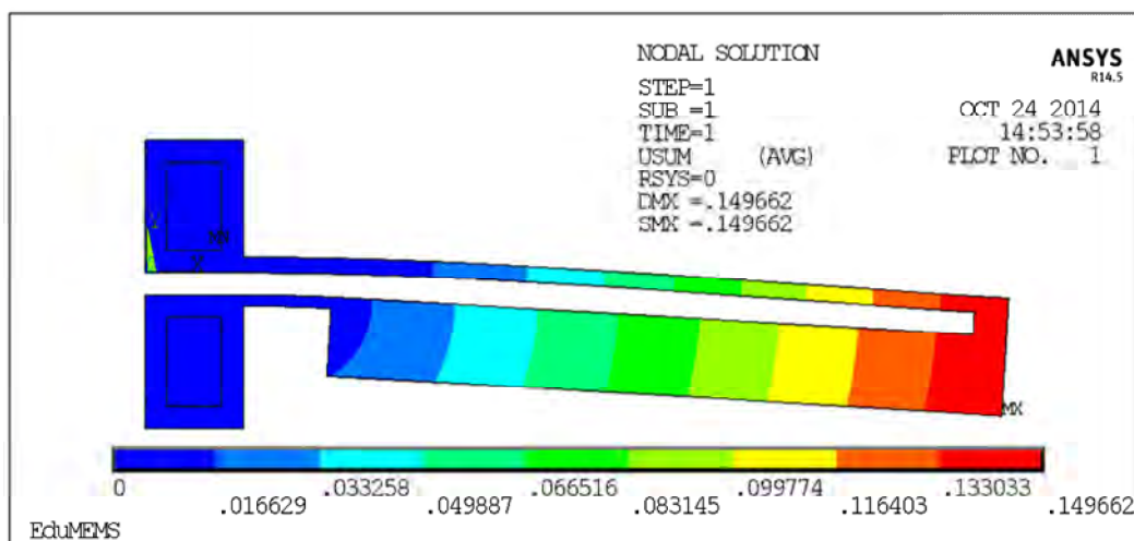
Fig. 10. The maximum displacement
