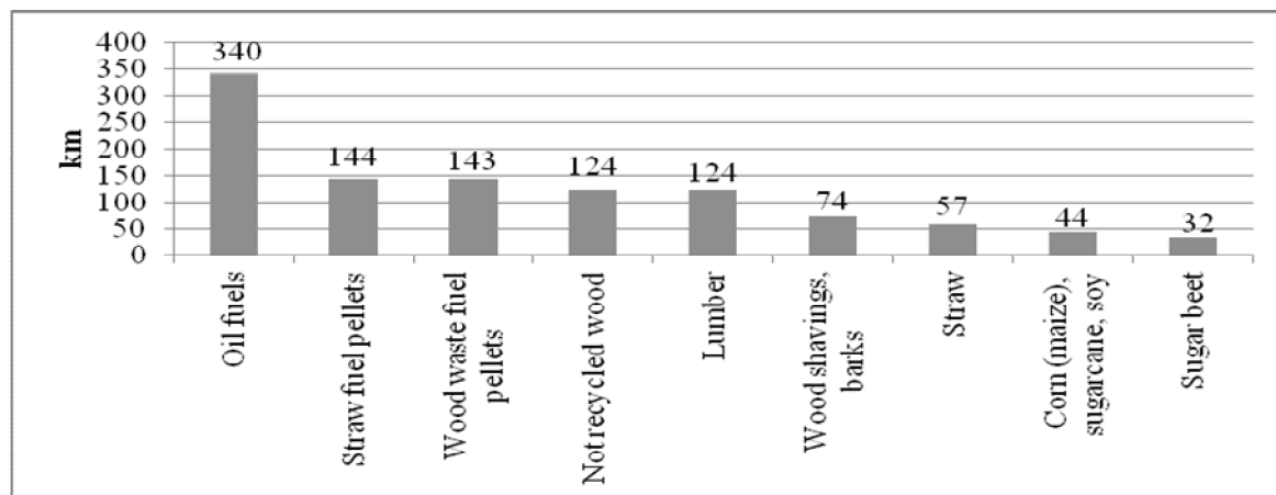
Fig. 2. The top distances of economically grounded transportation of different kinds of biomass [10]
