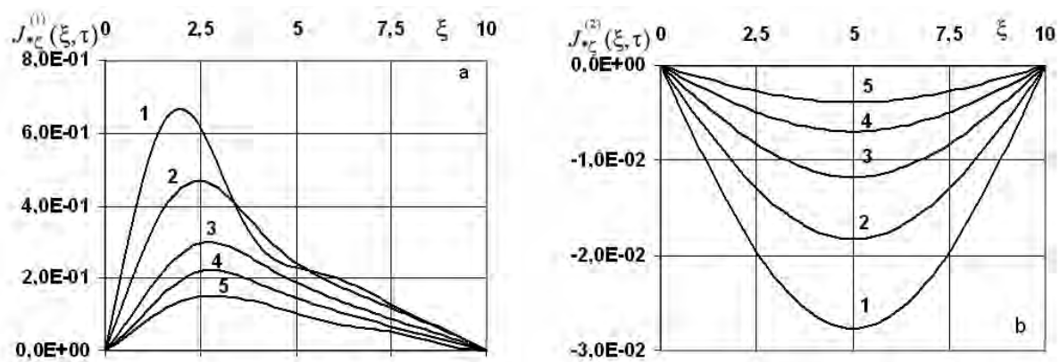
Fig. 7. Decaying particle flows J_{*ζ}^{(1)}(ξ, τ) in the middle of Ω_1 (a) and flows J_{*ζ}^{(2)}(ξ, τ) in the middle of Ω_2 (b) depending on the diffusion coefficient d .
