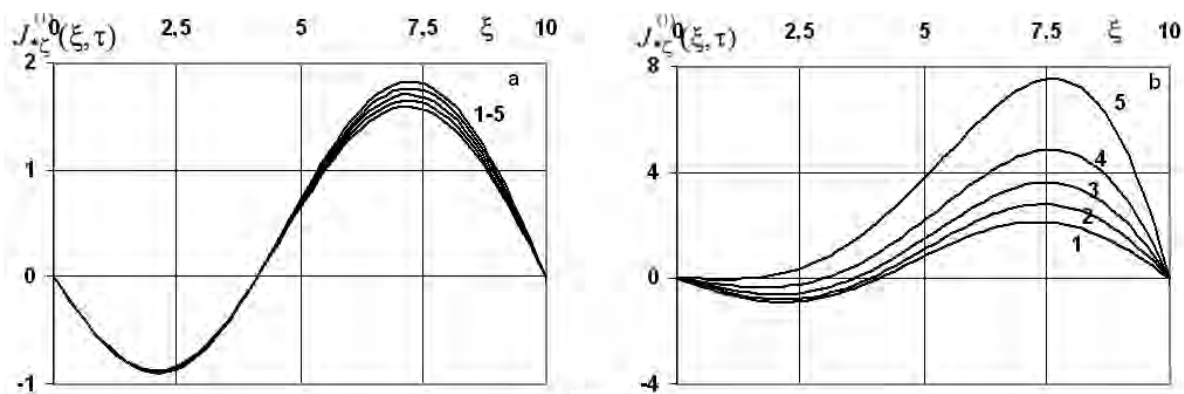
Fig. 3. Charts of decaying particle flows J_{*ζ}^{(1)}(\xi, \tau) in the middle of the thin channel depending on small (a) and large (b) values of the convective velocity \widehat{v} .
