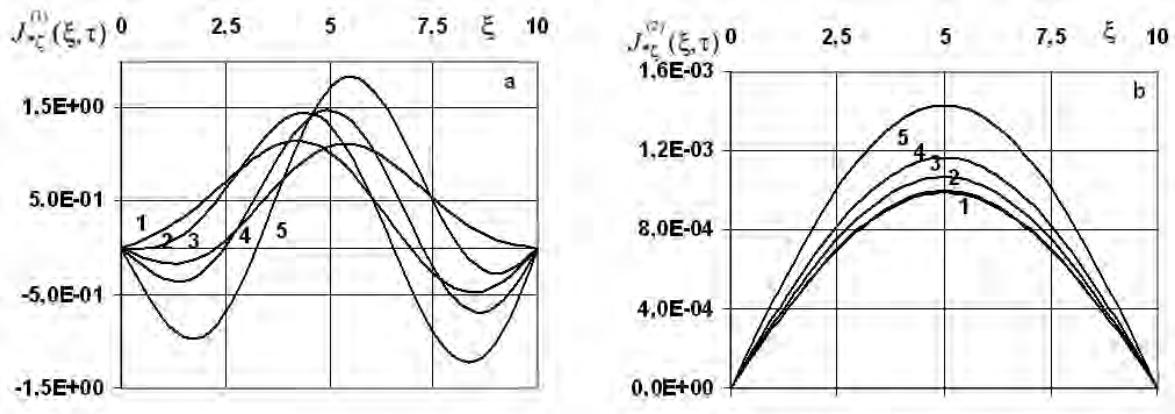
Fig. 6. Decaying particles flows J_{*ζ}^{(1)}(ξ, τ) in the middle of Ω_1 (a) and flows J_{*ζ}^{(2)}(ξ, τ) in the middle of Ω_2 (b) depending on the ratio of the coefficients of the concentration dependence of the chemical potentials η_1/η_2 .
