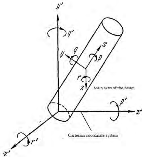
Fig. 2. Random placement of beams in space
