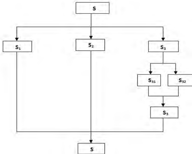
Fig. 1. Modeling complex systems by the diacoptic method
