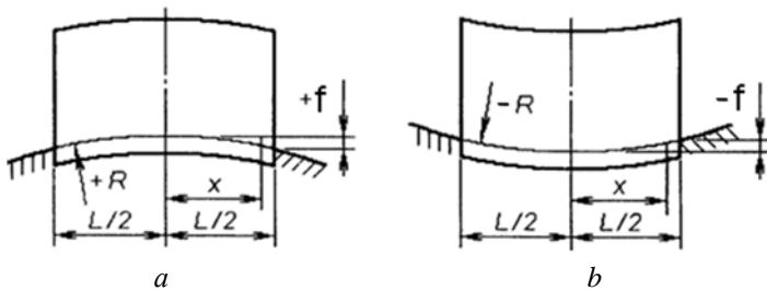
Fig. 3. Schemes of vertical displacements of bases under the foundations during the formation of the corresponding radiuses of curvature \pm R : a - sign "+" - convexity (curve); b - sign "-" -
