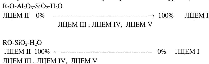
Fig.1. Principles chemе of alkaline cement type determination by the character of hydration products
