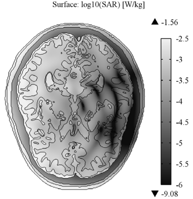
Fig. 7. SAR distribution in the developed human head phantom due to an incident plane wave propagating along x -axis (left-to-right).
