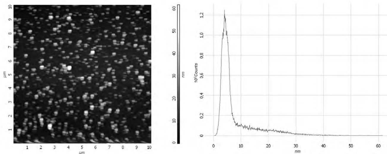
Fig. 2. AFM image of structures on the hydrophobic modified silicone surface 10 \times 10 \mu\text{m} (at the left). The distribution histogram in height of nanoparticles (at the right)
