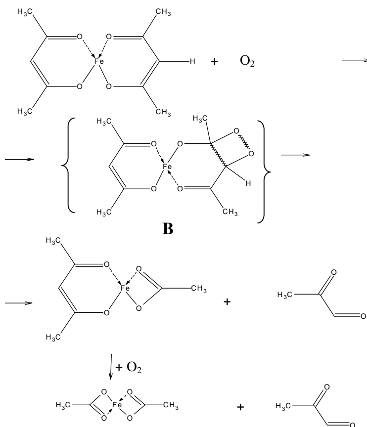
Scheme 2
