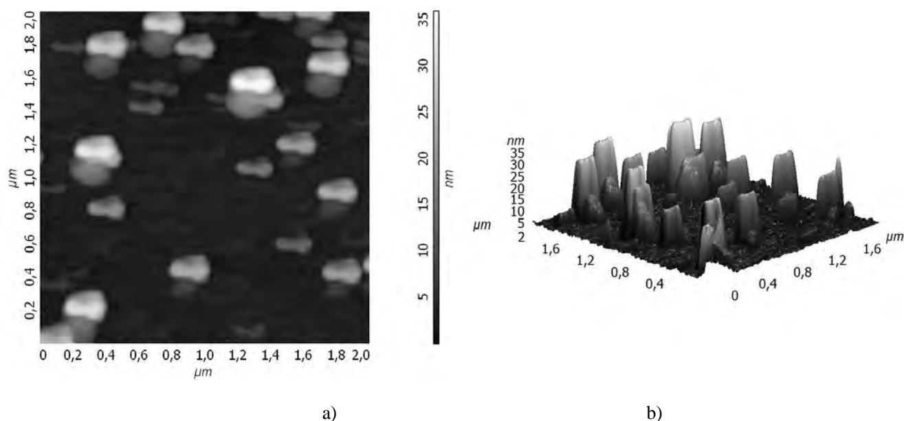
Fig. 1. The AFM two- (a) and three-dimensional (b) image of nanoparticles on the basis Ni_2(OAc)_3(acac) \cdot L^2 \cdot 2H_2O formed on the hydrophobic surface of modified silicone
