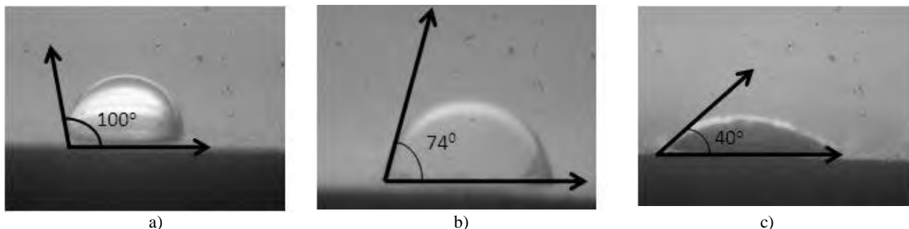
Fig. 6. Contact angle measurement for: pure zinc sheet (a); anodized film (b) and annealed film (c)
