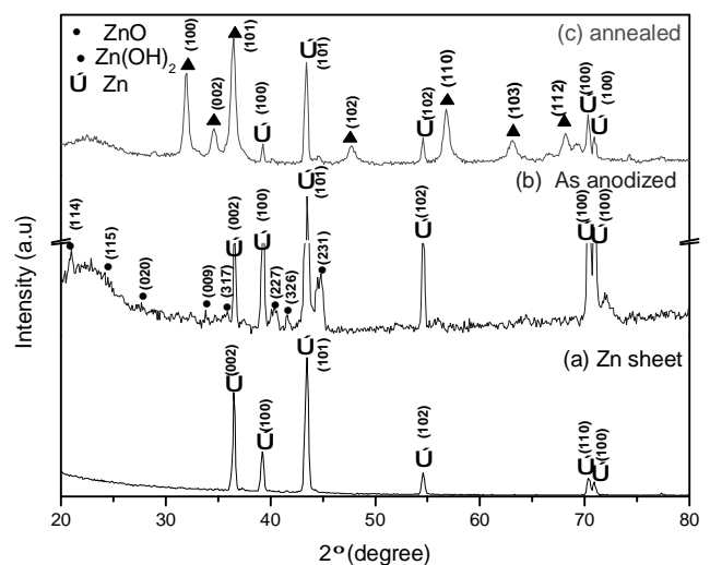
Fig. 2. X-ray diffraction pattern of zinc sheet (a); anodized film (b) and annealed film (c) at 523 K
