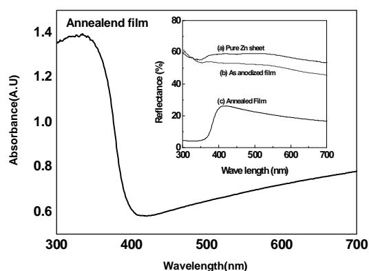
Fig. 5. Optical absorption spectra of annealed film (inset: reflectance spectra of pure Zn sheet (a); anodized film (b) and annealed film (c))
