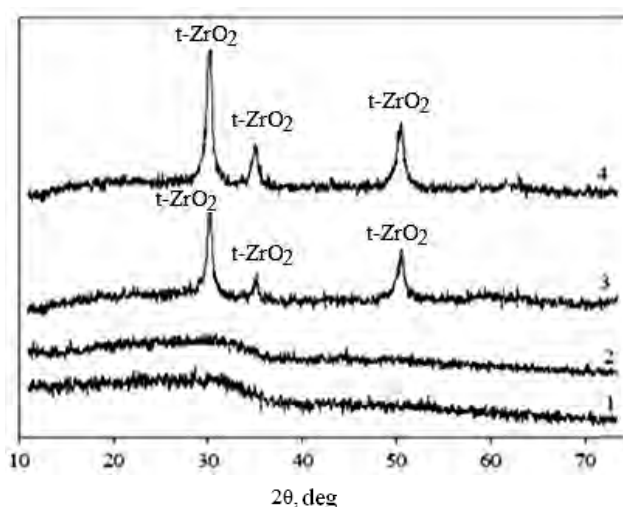
Fig. 1. X-ray diffractions of sample 1 treated at different temperatures, K: 573 (1); 623 (2); 673 (3) and 723 (4). t- \text{ZrO}_2 – tetragonal phase of zirconium(IV) oxide
