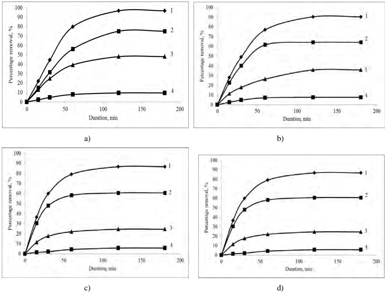
Fig. 3. The removal phosphates degree on the duration of sorption at different final temperatures treatment (K) of nanocomposites: 573 (1); 623 (2); 673 (3) and 723 (4). Sample 1 (a); Sample 2 (b); Sample 3 (c) and Sample 4 (d). Degree of phosphates sorption by crushed activated carbon at 120 min is 26.9 %
