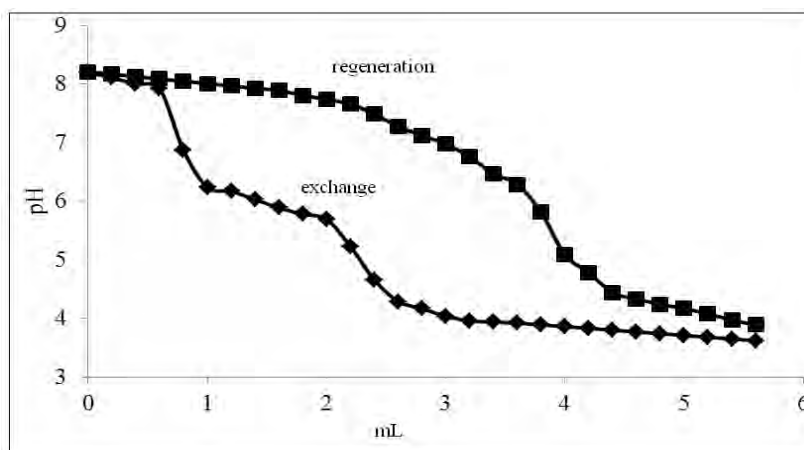
Fig. 4. Ion exchange and regeneration curves of nanocomposite Sample 1 synthesized by thermal treatment at 573 K
