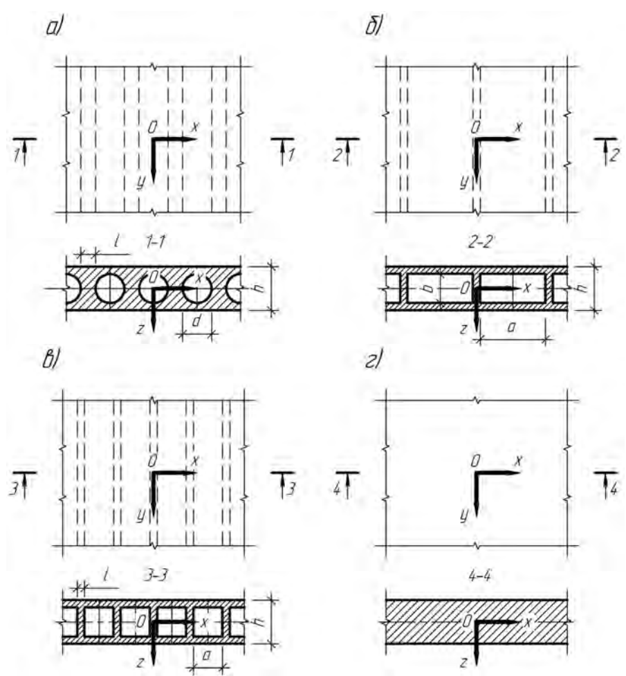
Fig.1. Actual (a, b, c) and calculated (d) Section monolithic slabs with tubular inserts
