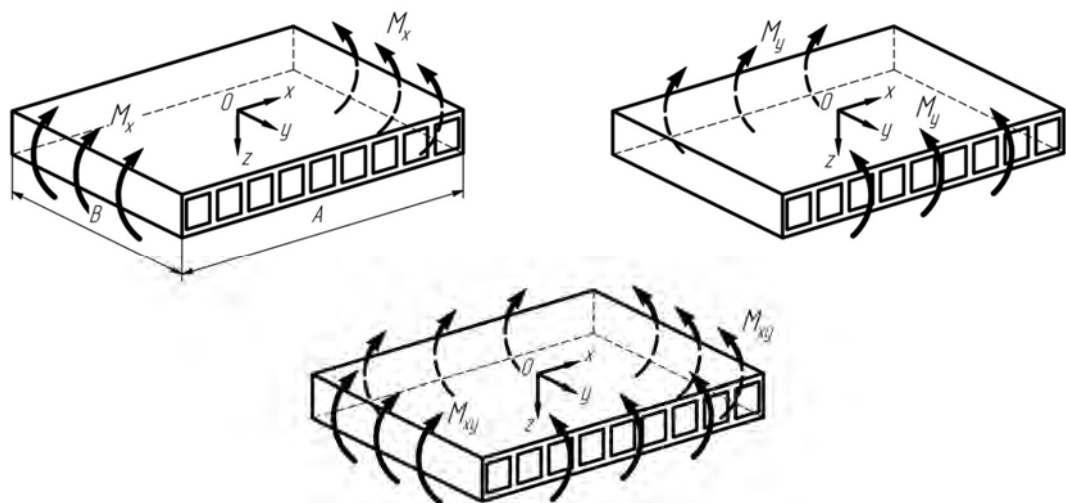
Fig. 2. Calculation of overlap with tubular inserts
