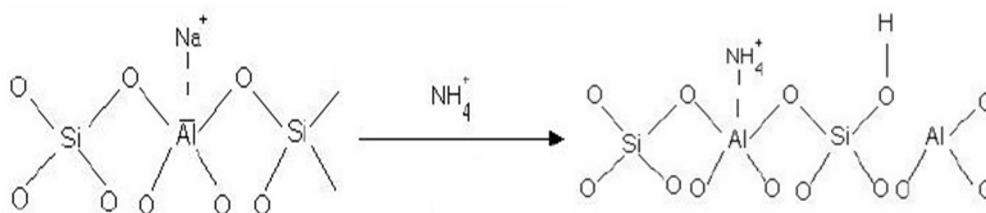
Fig.2. Scheme ion exchange of ammonium ion for sodium
