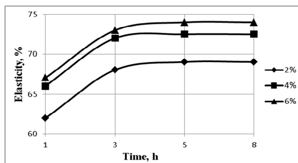
Fig. 5. Bitumen elasticity vs preparation time at different amounts of Butonal NS 104
