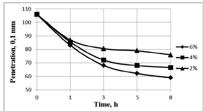
Fig. 1. Bitumen penetration at 298 K vs preparation time at different amounts of Butonal NS 104
