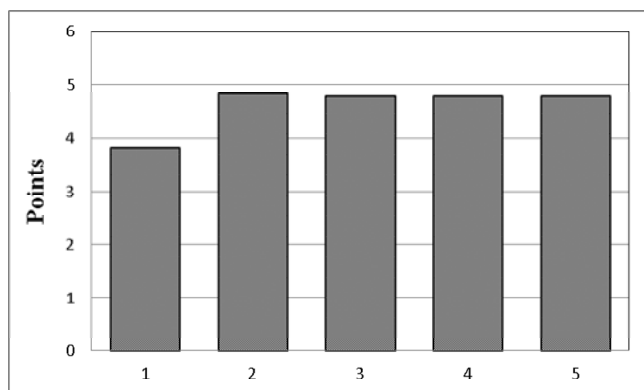
Fig. 7. Dependence of bitumen cohesion with mineral matter on the amount of modifier Butonal NS 198 (%): 0 (1); 2 (2); 3 (3); 4 (4) and 6 (5)
