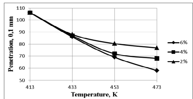
Fig. 2. Bitumen penetration at 298 K vs preparation temperature at different amounts of Butonal NS 104
