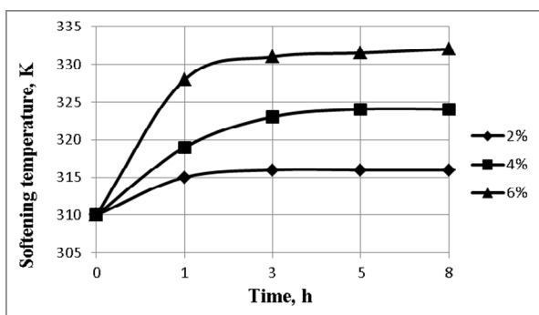
Fig. 3. Softening temperature vs preparation time at different amounts of Butonal NS 104
