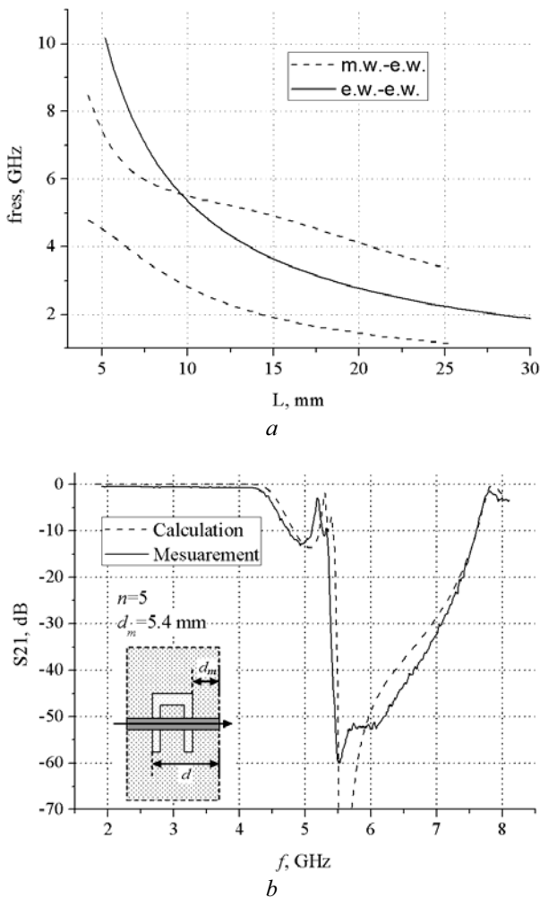
Fig. 5. The characteristics of the microstrip resonator with symmetric \Pi -shaped slot, Fig 1b: (a) eigenfrequency spectrum, and (b) insertion losses of 5-cell periodic structure. The resonator parameters (in mm): screen dimensions b_1=b_2=12.0 , A=24.0 ; slot resonator dimensions: 2a=4.4 , b=2.2 , s_1=s_2=0.5 .
