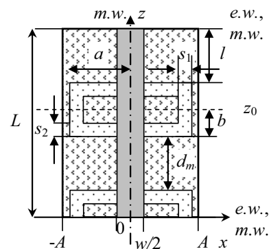
Fig. 6. 3-cell periodic structure: the topology of the resonator for the boundary problem to solve.
