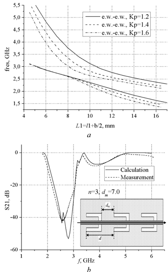
Fig. 4. The characteristics of the microstrip resonator with nonsymmetric \Pi -shaped slot, Fig 1a: (a) eigenfrequency spectrum, and (b) insertion losses of 3-cells periodic structure. The resonator parameters (in mm): substrate h=1.0 , \epsilon_{r1}=9.8 , the microstrip line width w=1.0 (characteristic impedance Z_0=50 Ohm), screen dimensions b_1=9.0 , b_2=5.0 , A=24.0 , slot resonator dimensions: a=8.0 , b=8.0 , s_1=0.5 , s_2=0.75 .
