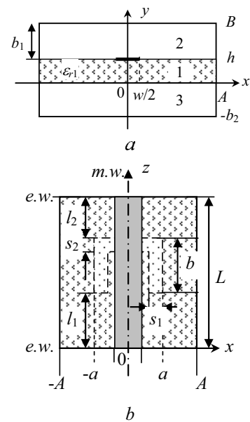
Fig. 2. Topology of the boundary problem: cross section (a) and top view (b) of the microstrip resonator with non-symmetrically located II-shaped slot discontinuity in the ground plane.
