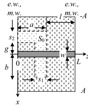
Fig. 3. Topology of the boundary problem of the microstrip resonator with symmetrically located \Pi -shaped slot discontinuity in the ground plane.
