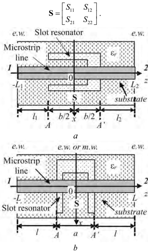
Fig. 1. II-shaped slot resonator in the microstrip line ground plane: (a) non-symmetric and (b) symmetric discontinuity.
