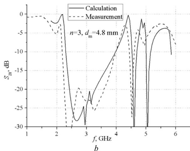
Fig. 7. The characteristics of the 3-cell periodic structure with symmetric O-shaped slot resonators in the microstrip line's ground plane: (a) eigenfrequency spectrum, and (b) insertion losses of the structure. Dimensions of the O-shaped slot resonator (in mm): a=12.9 , b=2.15 , s_1=s_2=0.5 .
