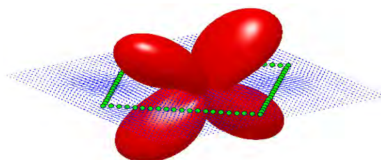
Fig. 13. Radiation pattern at the frequency of 2.8 GHz, horizontal polarization.
