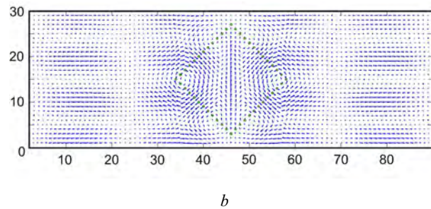
Fig. 3. The distribution of surface currents of the slot in vertical (a) and horizontal (b) screens.
