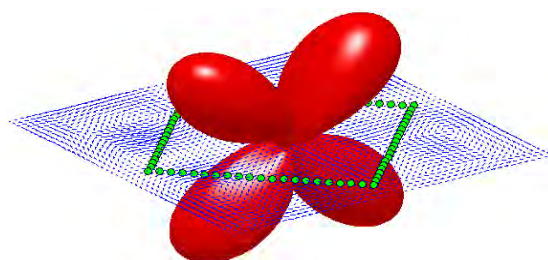
Fig. 14. Radiation pattern at the frequency of 3.4 GHz, horizontal polarization.
