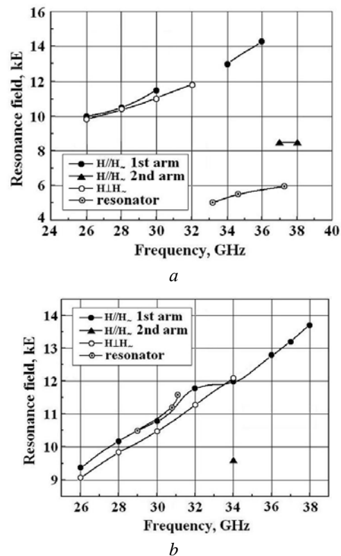
Fig. 4. A spectrum of magnetic resonance for the nanocomposite sample, containing manganese-zinc-ferrite (a) and nickel-zinc-ferrite (b).
