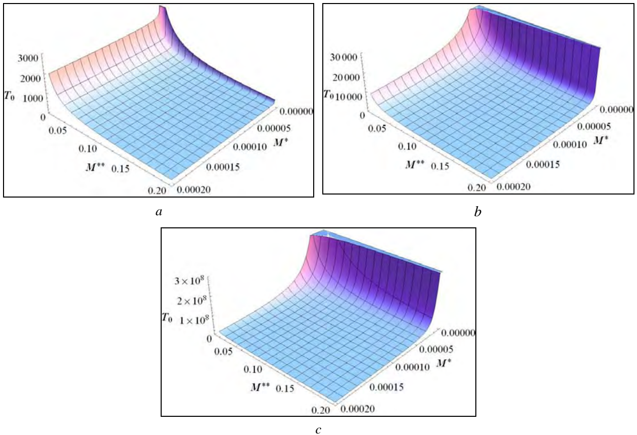
Fig. 1. Dependence of the value T_0 on generalized parameters of the oscillating system under various values of the exponent p
