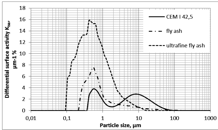
Fig. 3. Coefficient of differential surface activity K_{sa} of materials
