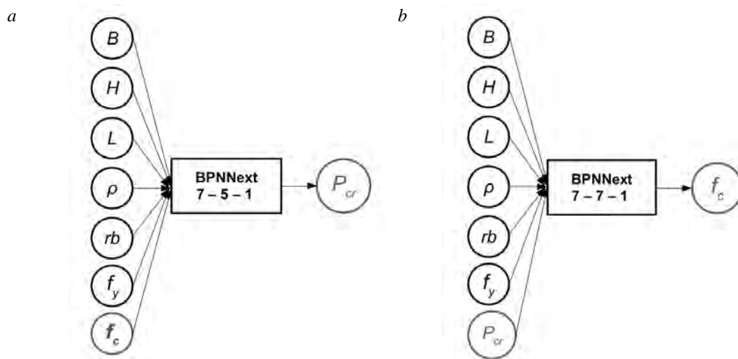
Fig. 1. BPNNext for: a) Prediction of critical load P_{cr} , b) Identification of concrete strength f_c
