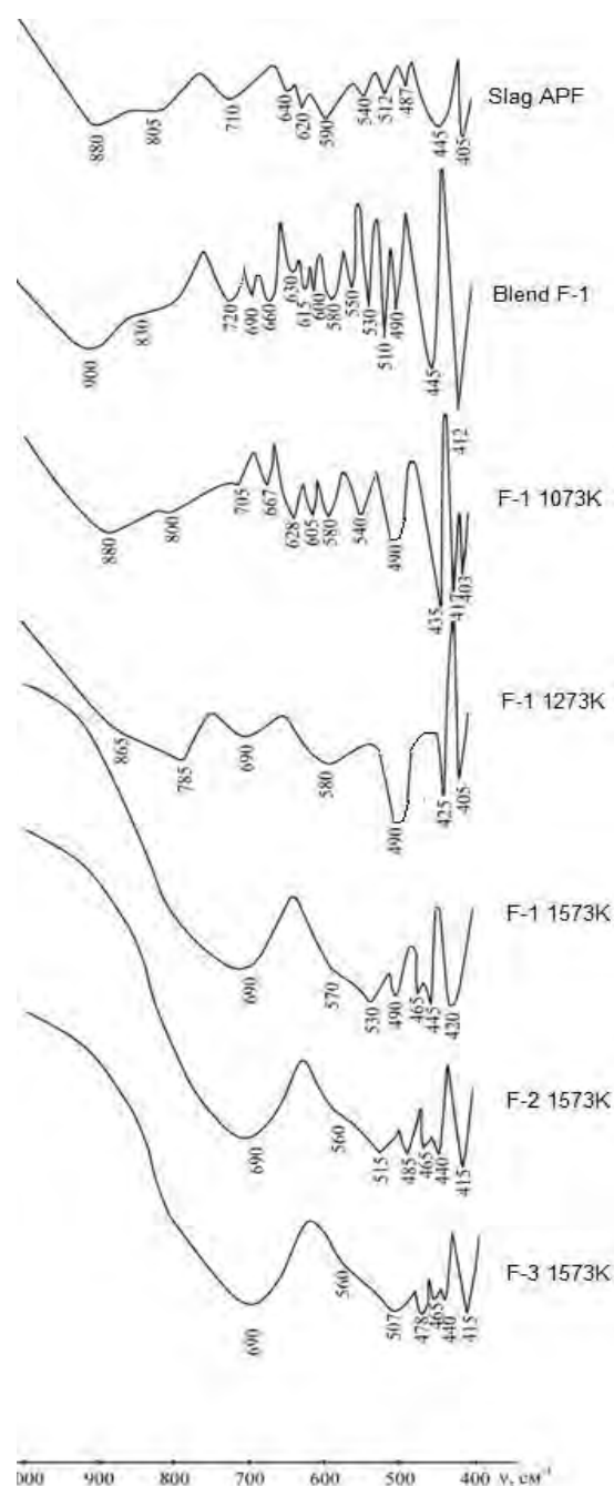
Fig. 4. IR-spectra of ceramic pigments (F-1)–(F-3), obtained at different temperatures
