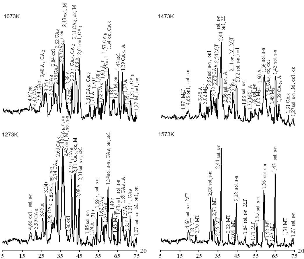
Fig. 3. Diffractograms of ceramic pigment F-1, baked in the temperature range of 1073–1573 K: A – \alpha - \text{Al}_2\text{O}_3 ; \text{CA}_6 – \text{CaO} \cdot 6\text{Al}_2\text{O}_3 ; \text{CA}_2 – \text{CaO} \cdot 2\text{Al}_2\text{O}_3 ; r – \text{TiO}_2 (rutile); sol. s-n – solid solution between \text{CoAl}_2\text{O}_4 and \text{MgAl}_2\text{O}_4 ; \text{M}_2\text{T} – \text{Mg}_2\text{TiO}_4 ; MT – \text{MgTiO}_3 ; ok – CoO; ok1 – \text{Co}_3\text{O}_4 ; M – MgO
