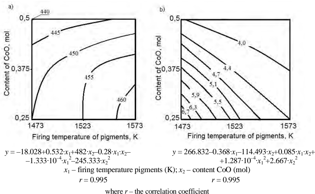
Fig. 5. Influence of the temperature of firing and concentration of cobalt oxide in the research of ceramic pigments on the length of wave (a) and the ratio of diffuse reflection (b) glaze of the coatings obtained with their introduction
