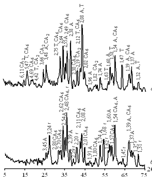
Fig. 1. X-ray phase analysis of researched slag: initial (a) and after thermal processing at 1573 K (b). A – \alpha\text{-Al}_2\text{O}_3 ; T – \text{TiO} ; \text{CA}_6 – \text{CaO}\cdot 6\text{Al}_2\text{O}_3 ; \text{CA}_2 – \text{CaO}\cdot 2\text{Al}_2\text{O}_3 ; r – \text{TiO}_2 (rutile)
