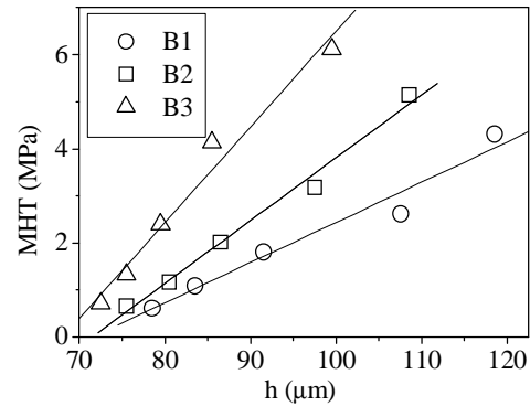
Fig. 9. Total microhardness plotted vs. indentation depth h
