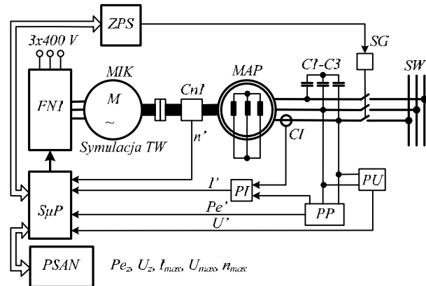
Fig. 4. Laboratory model of small hydro-electric power plant, connected to isolated grid and simulated by cage induction motor supplied from frequency converter and mounted on common shaft with slip-ring induction machine having rotor windings short-circuited.
