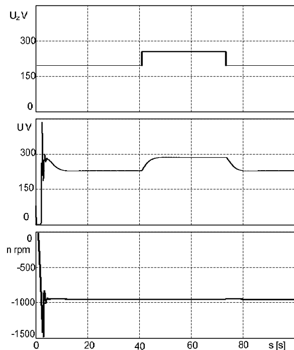
Fig. 6. Output voltage U and speed n waveforms in closed-loop control system NMAK as response to change in set voltage U_z
