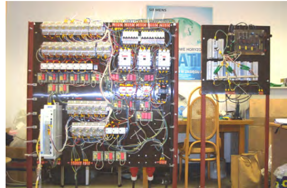
Fig. 5. Control panel and frequency converter – test stand
