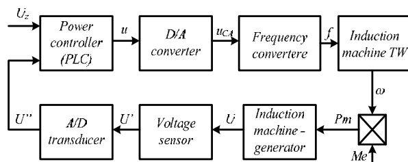
Fig. 1. Schematic diagram of voltage control system in MAP stator circuit; MAP operates as generator and is driven with cage asynchronous machine supplied via frequency converter and simulating a water turbine
