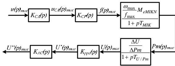
Fig. 3. Block diagram of open-loop MAP stator rms voltage control system; MAP machine operates as generator within isolated grid and is driven with MIK machine supplied via frequency converter and simulating a water turbine
