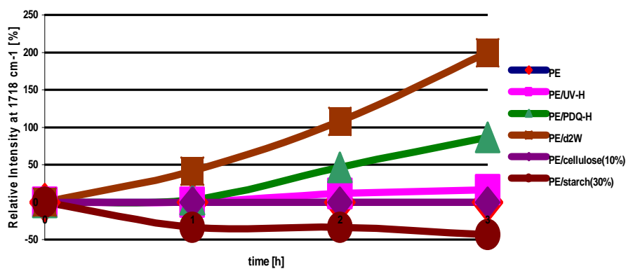
Fig. 6. Relative intensity in FT-IR at the ketone carbonyl band (appr. 1718\text{ cm}^{-1} ) during oxidation on air at 363 K
