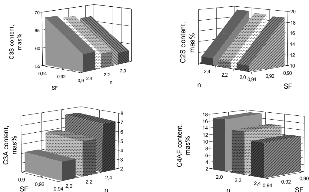
Fig. SF and n influence on the content of the main clinker minerals
