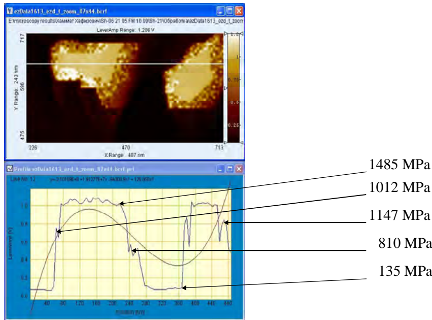
Fig. 1. The processed in SPIP image of nanocomposite butadiene-styrene rubber/nanoshungite, obtained by force modulation method, and mechanical characteristics of structural components by the data of nanoindentation (strain 150 nm)
