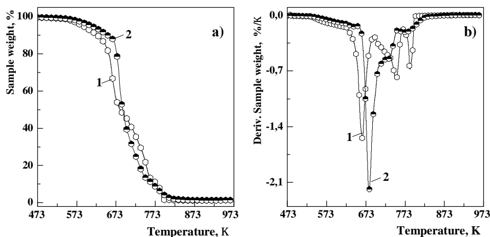
Fig. 7. The TGA (a) and DTG (b) data for TPE based on HDPE/EPDM/GTR/Bitumen (40/35/12.5/12.5) irradiated by \gamma -rays (1) and e -beam with the dose of 100 kGy (2)
