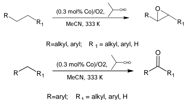
Scheme 1. Hydrocarbons oxidation with CoCl 2 and Co(CH 3 COO) 2 immobilized in polyaniline matrix
