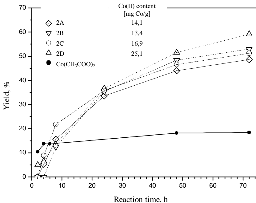
Fig. 2. Dec-1-ene oxidation on PANI immobilized with Co(CH 3 COO) 2 at 298 K (2A-2D)
