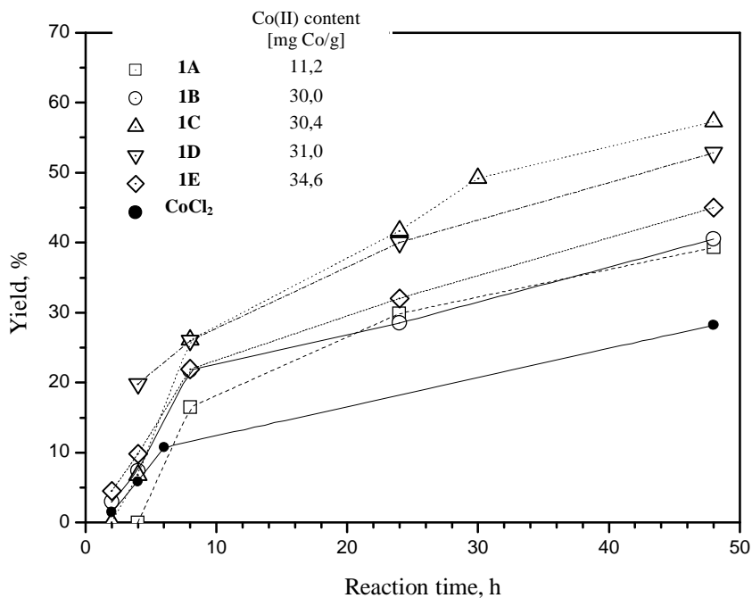
Fig. 1. Dec-1-ene oxidation on PANI immobilized with CoCl 2 at 298 K (1A-1E)
